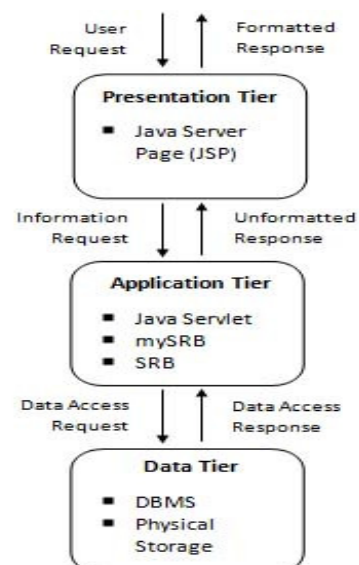
Figure 3. The architecture and interaction cycle of GREET.
