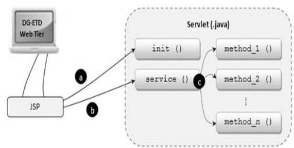
Figure 6. The java servlet request interaction.
