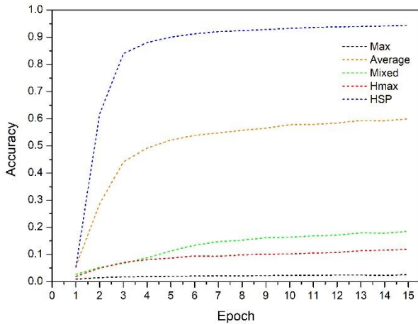
Figure 7. Convergence plot of training accuracy.
