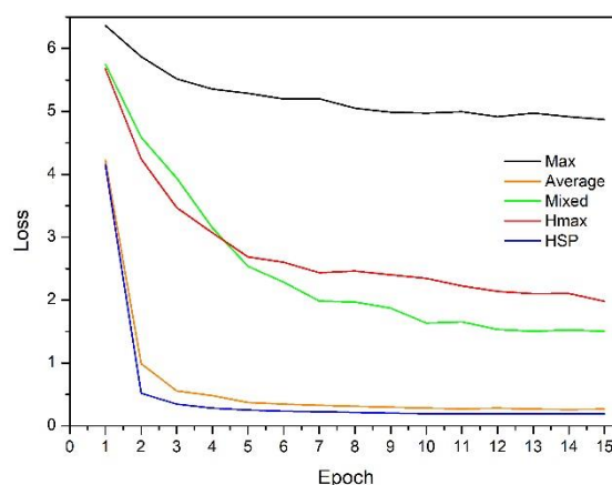
Figure 6. Convergence plot of validation loss.
