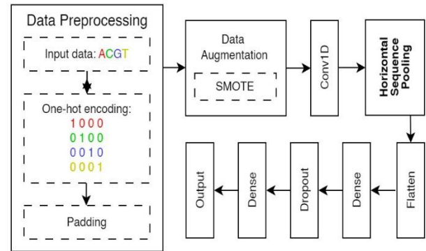
Figure 4. The overall model with HSP.
