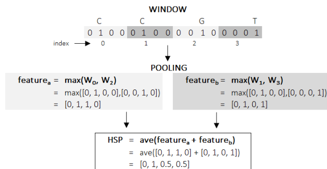
Figure 3. Example of HSP operation.
