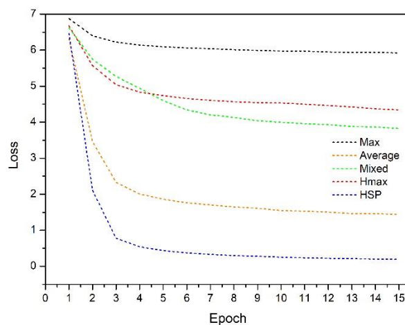
Figure 5. Convergence plot of training loss.
