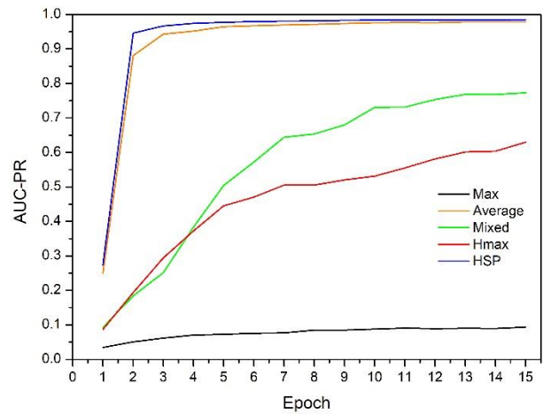
Figure 10. Convergence plot of validation AUC-PR.
