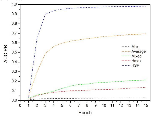
Figure 9. Convergence plot of training AUC-PR.
