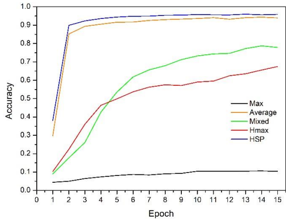
Figure 8. Convergence plot of validation accuracy.
