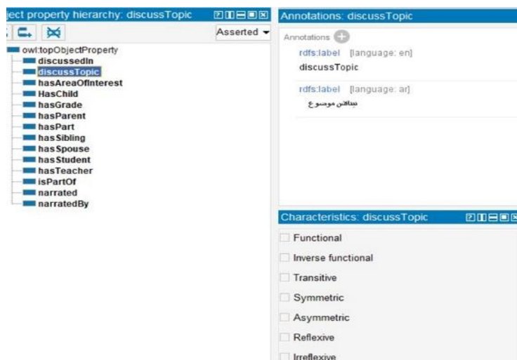
Figure 3. We defined the object properties of OntoHadith.
