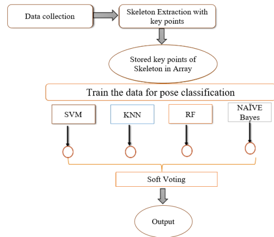
Figure 3. Methodology for activity recognition.
