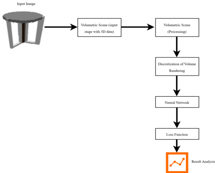
Figure 2. Process steps for NeRF.
